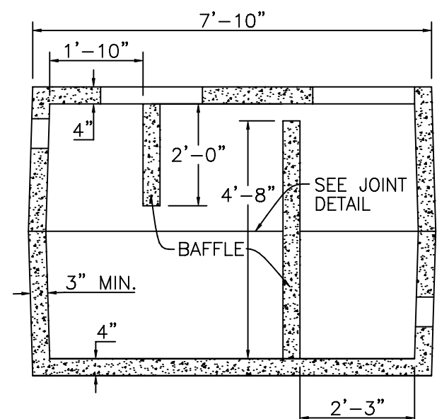
LONG SECTION
