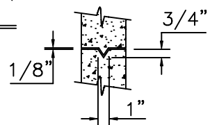
JOINT DETAIL
