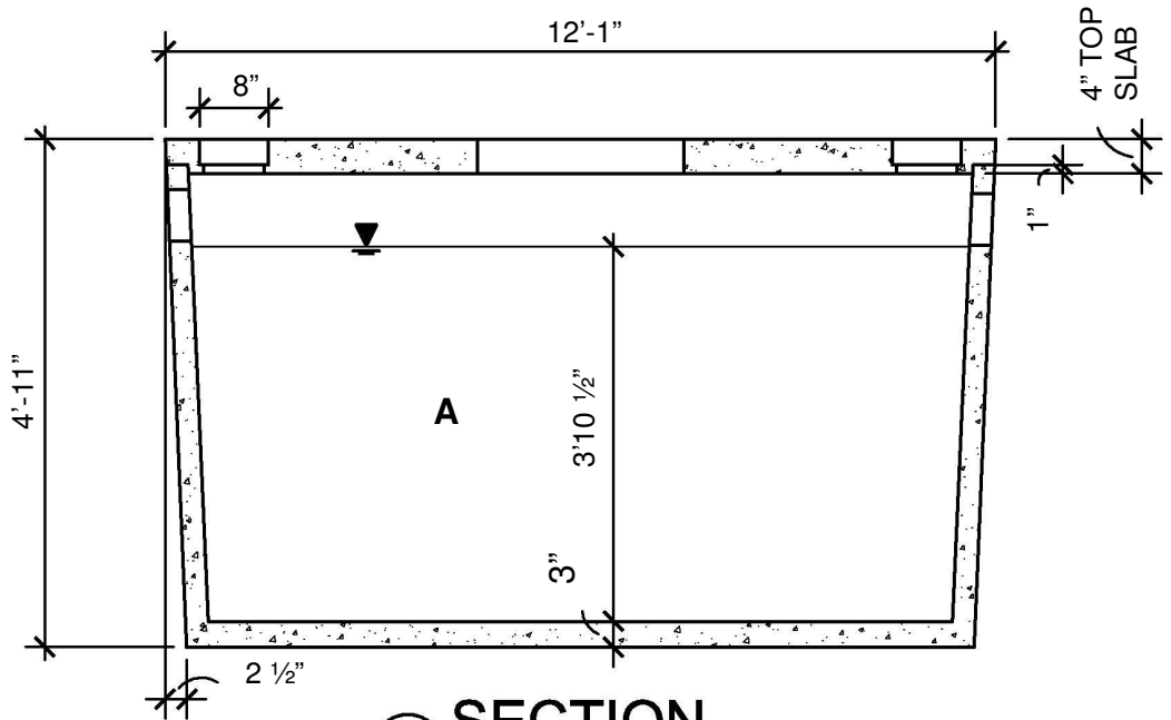
1 SECTION 1/4" = 1'-0"
