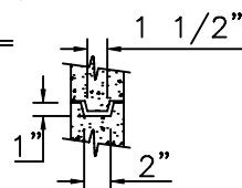
JOINT DETAIL
