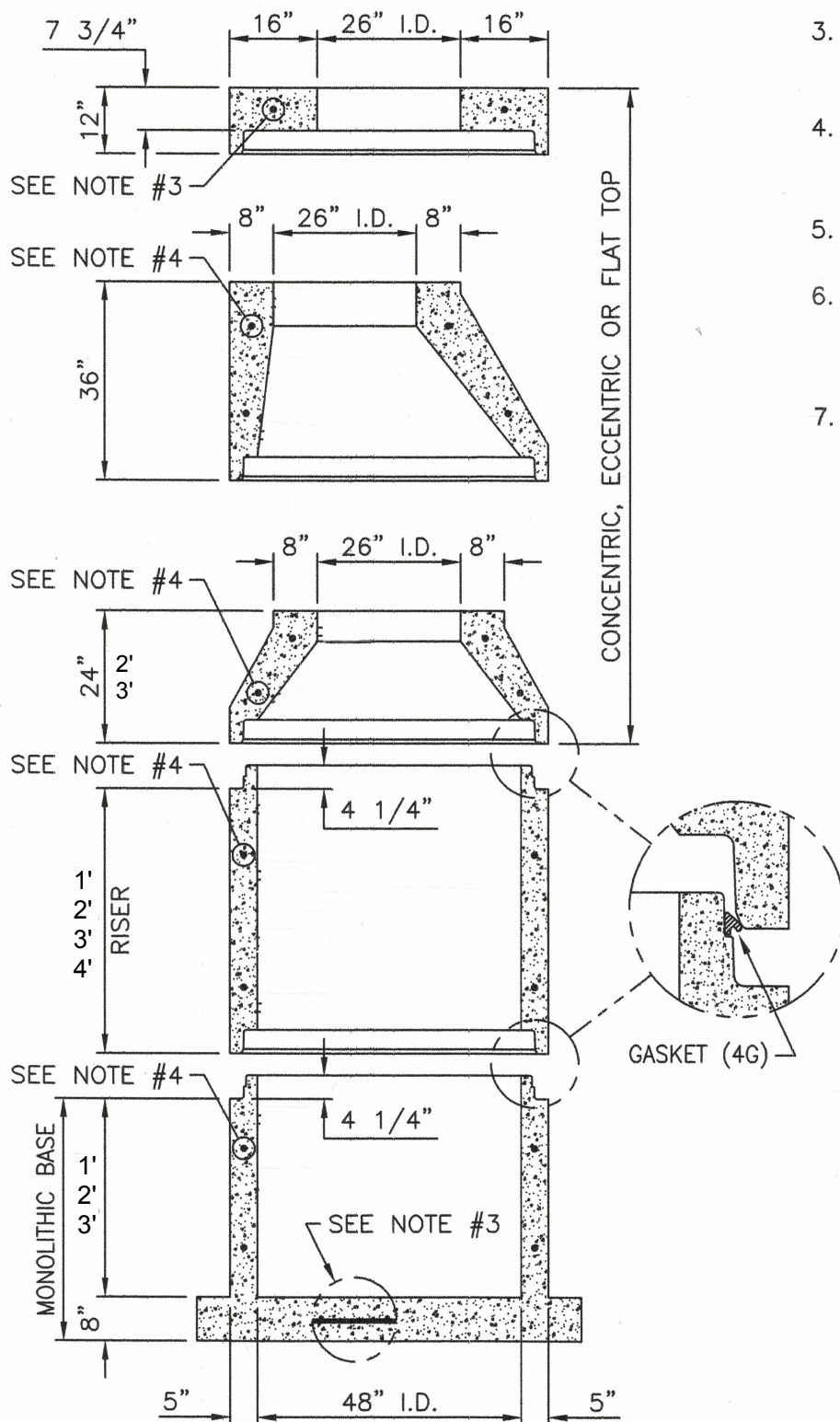
MANHOLE ASSEMBLY
