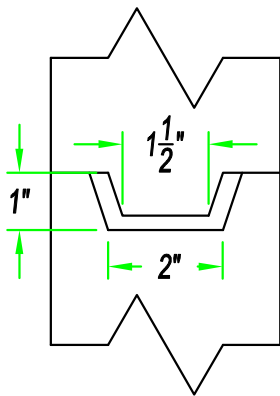
Joint Detail
